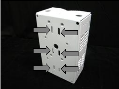
Image 1) Center Slots for strapping Start strapping from rear, this view show slot arrows shown on face
