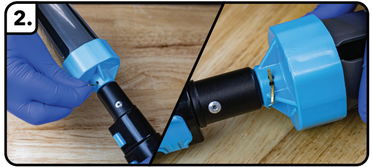
2. Place supplied cotter pin through the small head base and bend tines away.
